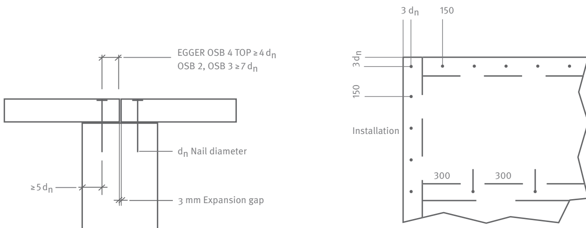
Fastening recommendations for non-load-bearing sheathing made of EGGER OSB
