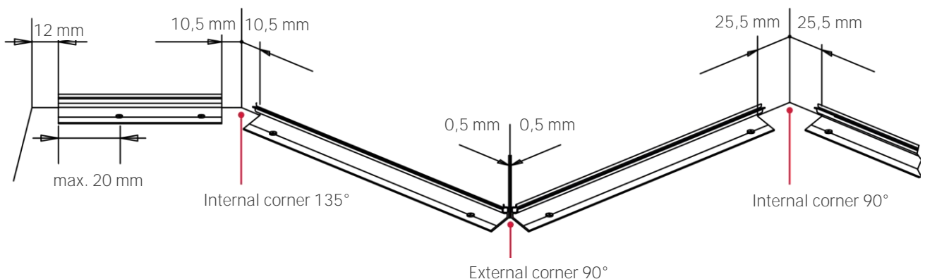
Base profile
