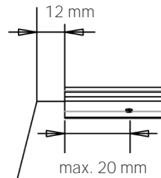
Fixing dimensions base profile
