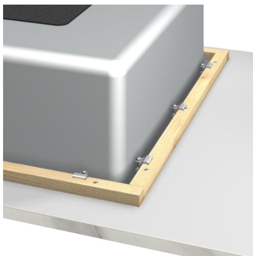
Fig. 1 – PerfectSense Topmatt worktop with edging
