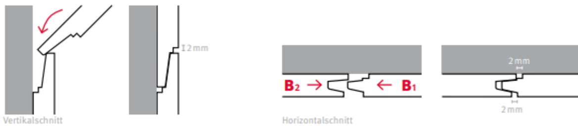
Figure 2: Edge profiling with automatically formed 2mm expansion joint
