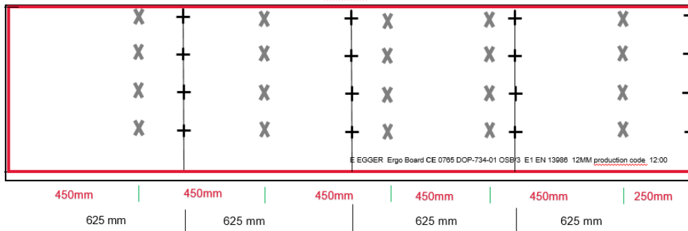
Figure 4: Nail grid print on the panel surface
