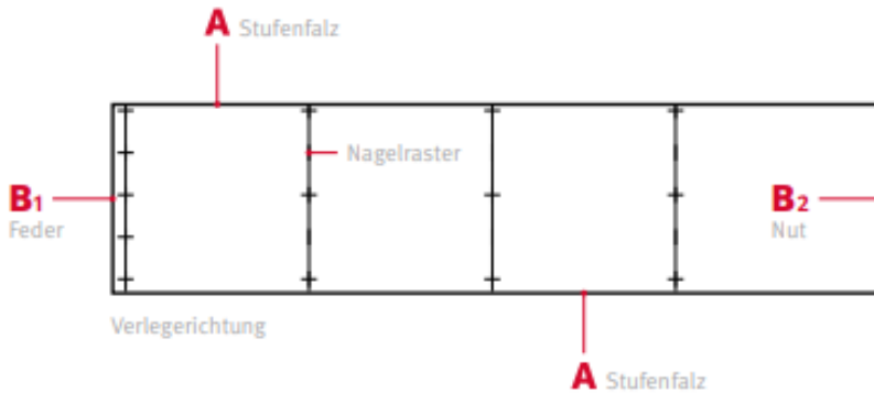
Figure 2: Edge profiling with automatically formed 2mm expansion joint
