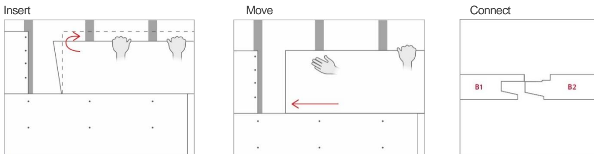
Figure 3: Installation of Ergo Board
