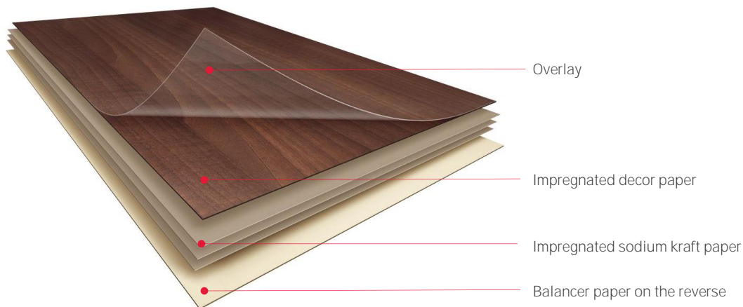
Laminate structure MED – Nominal thickness 0.031 inch (0.80 mm)
